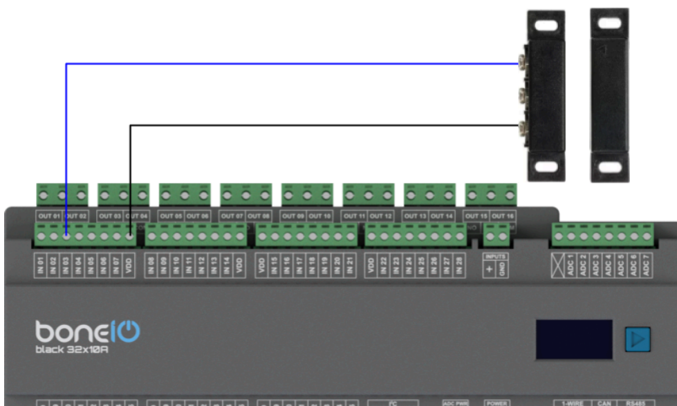
Connecting reed switch.
